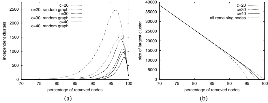
Fig. 8. Partitioning of the communication graph as a function of the percentage of removed random nodes (node failures). The curves belong to a single graph. The largest clusters of random graphs are omitted for clarity; their relationship to the communication graphs is similar to the relationship in the case of the number of clusters.
