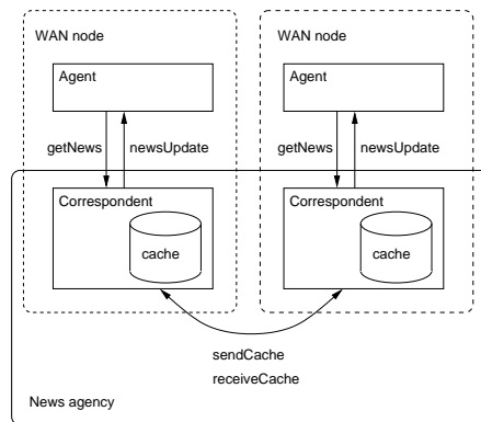
Fig. 1. The organization of a newscast application.
