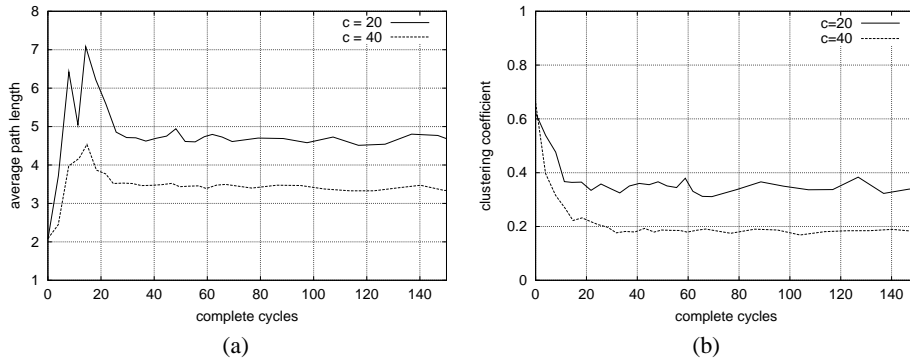
Fig. 6. (a) The evolution of average path length from a node. (b) Clustering coefficient.
