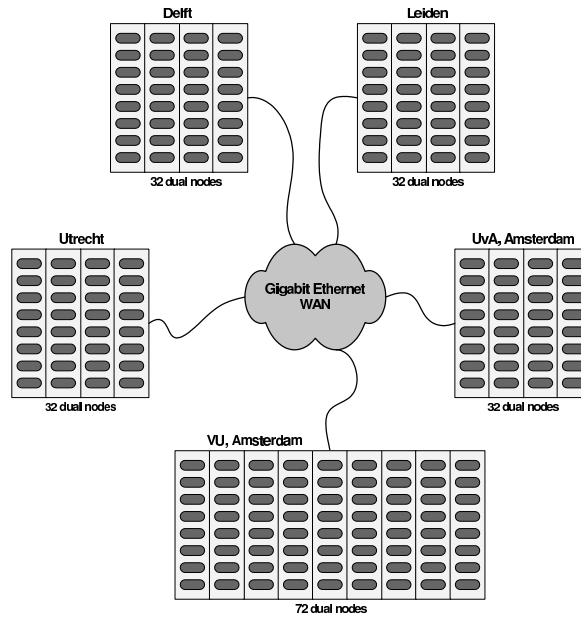
Fig. 5. The DAS-2 architecture
