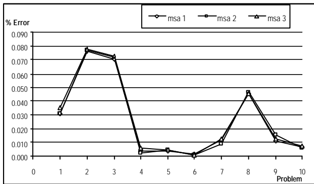
Figure 3; error percentage of found results respecting each migration rate.
