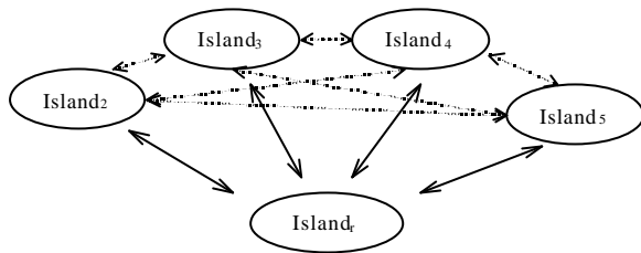
Figure 2; inter-islands relationships for parallel MSA
